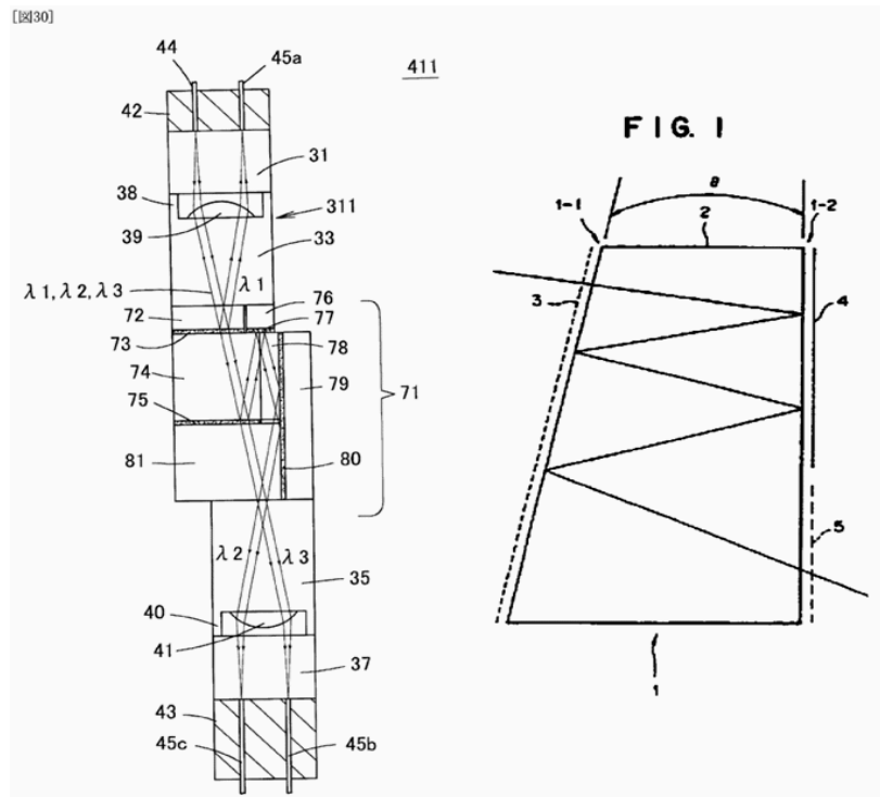
Zigzag path in solid block formed of components 74,78,81 and single solid block 2 (Sources WO2006080249 for fig. 30, GB2304204 for fig. 1).
