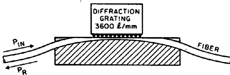
Fig. 1. Cross section schematically showing metallic grating in contact with polished fiber.
