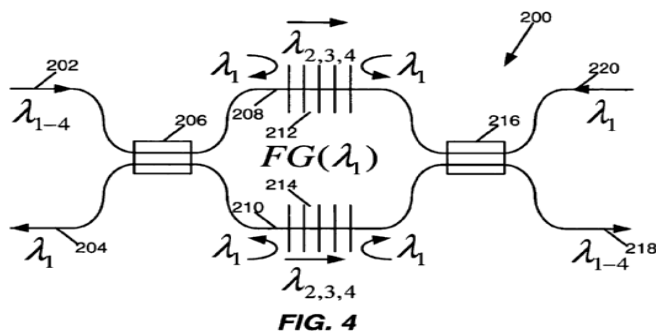
Gratings 212 & 214 in arms 208 & 201 of Mach-Zehnder Interferometer. (Source US2006002653).
